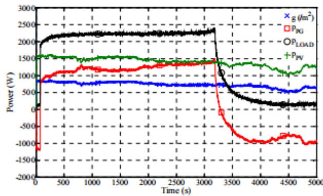
Figure 9. Solar irradiance g evolution on March 10 th in 2010 starting from 30 pm at Compiègne and EV charging system powers evolutions ( p_{PV} applied by PV system versus g solar irradiance, p_{LOAD} absorbed by BEV, and p_{PG} for public grid).
