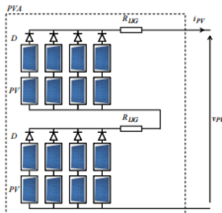
Figure 3. PV panels electrical coupling.
