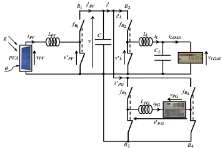
Figure 4. BEV charging electrical scheme.
