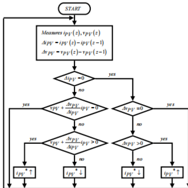
Figure 5. Flow chart of the INC algorithm.
