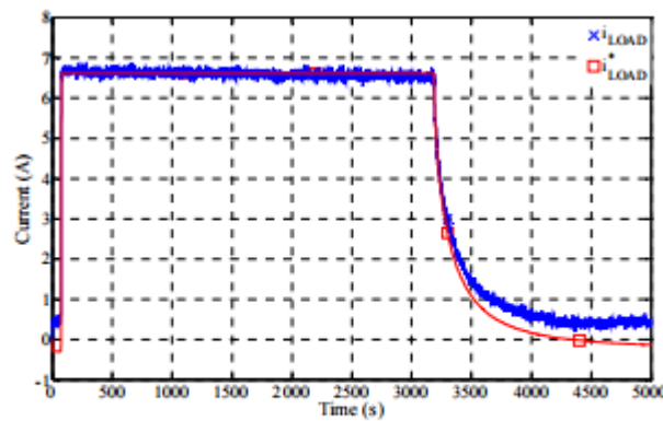
Figure 6. BEV current mode charge.
